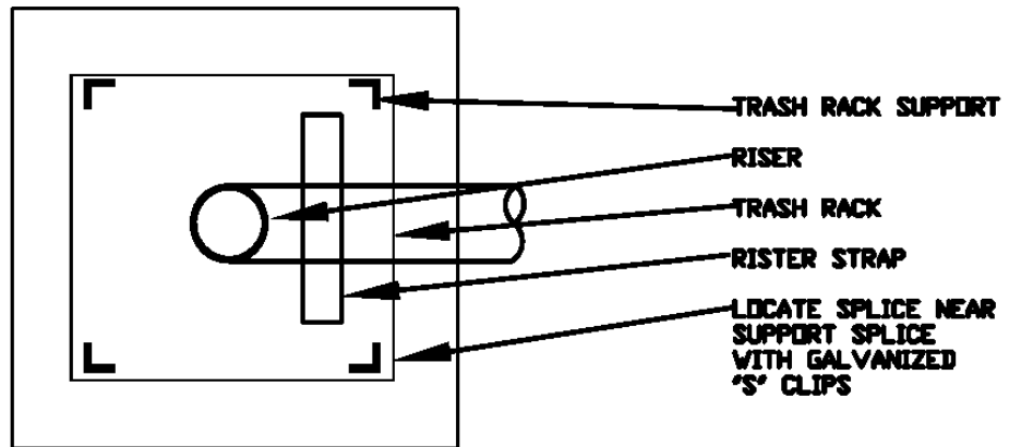
Top View of Riser (Square Design)
